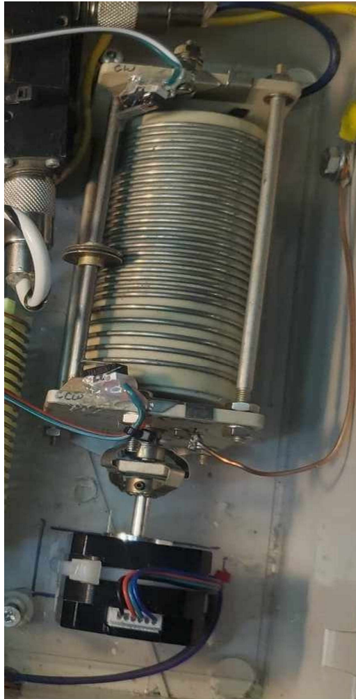
Figure 11 – Notice the isolation coupler now installed between the motor and the inductor.
