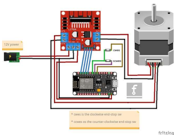
Figure 4 – Wiring diagram.
